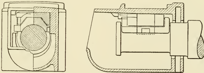
Fig. 19. Journal Box with Journal and Bearing in Position
